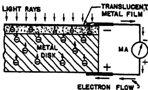
Basic construction of photovoltaic cells.
